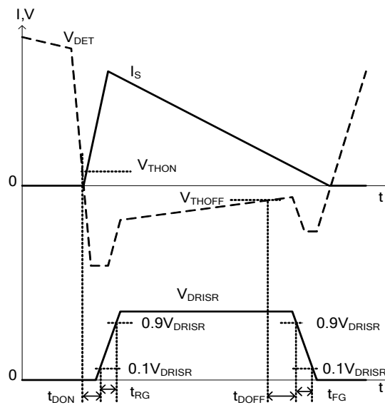
Figure 2. Typical Waveforms of APR34330
