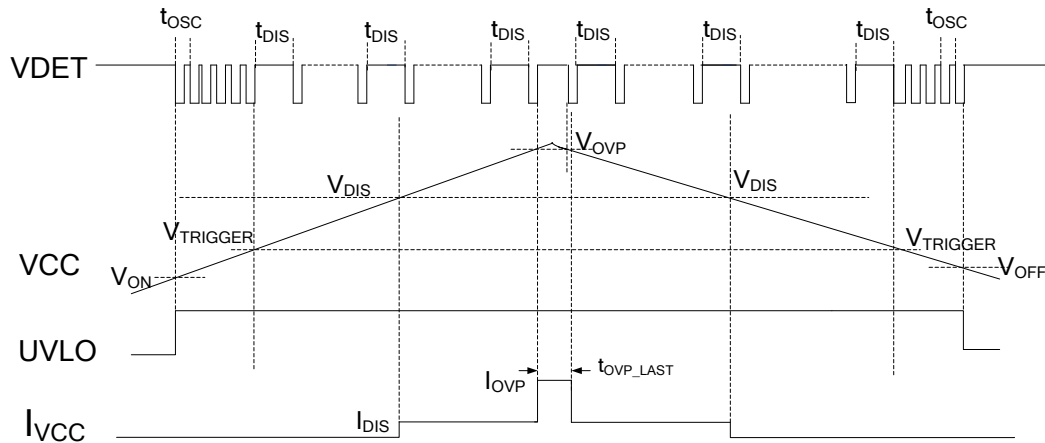
Figure 1. Typical Waveforms of APR34330
