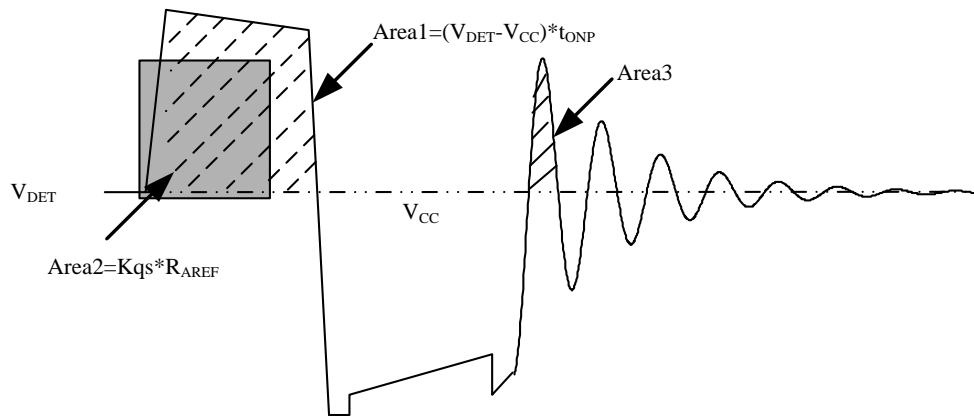
Figure 3. AREF Function
